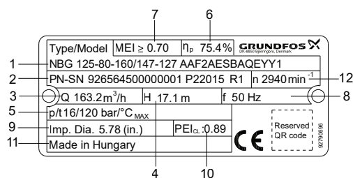
Example of NB, NBE nameplate
