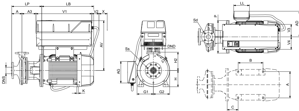
Mounting design B
