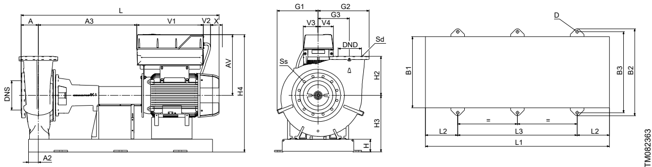
EN/ISO base frame with 6 mounting holes, tangential outlet
