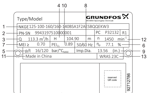
Example of NK, NKG nameplate
