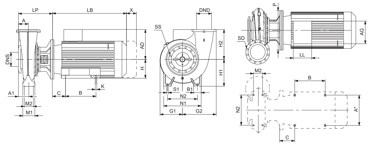
Mounting design C2, tangential outlet
