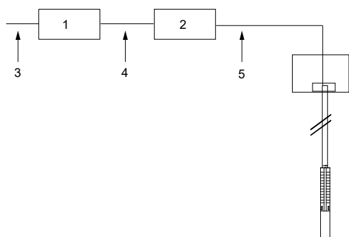
Example of installation in EMC-insensitive sites
