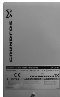
Motor starter for MS 402 and MS 4000
