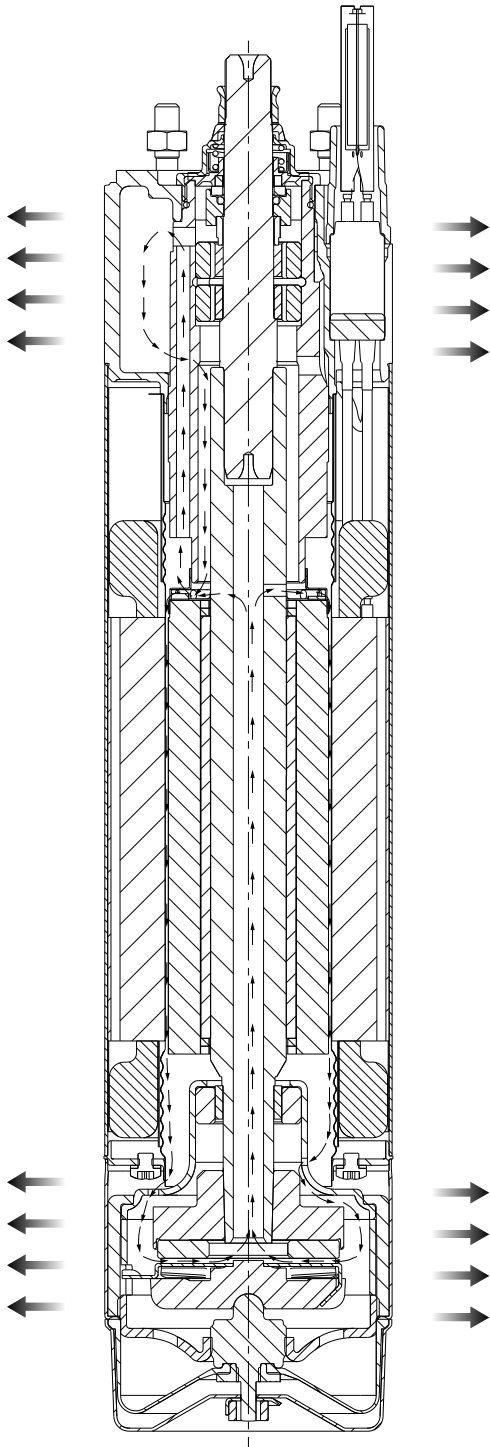
Internal circulation system for cooling
