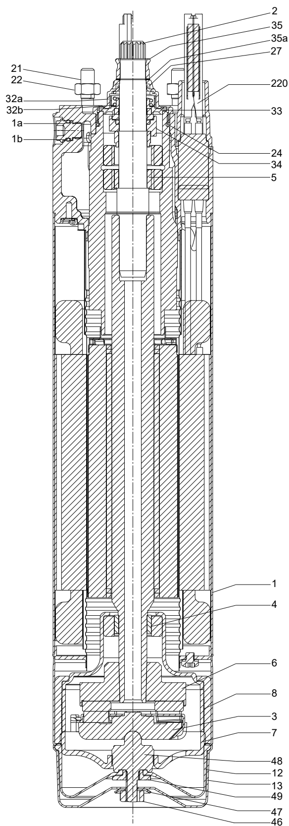
Sectional drawing of the MS4000 Model C motor
