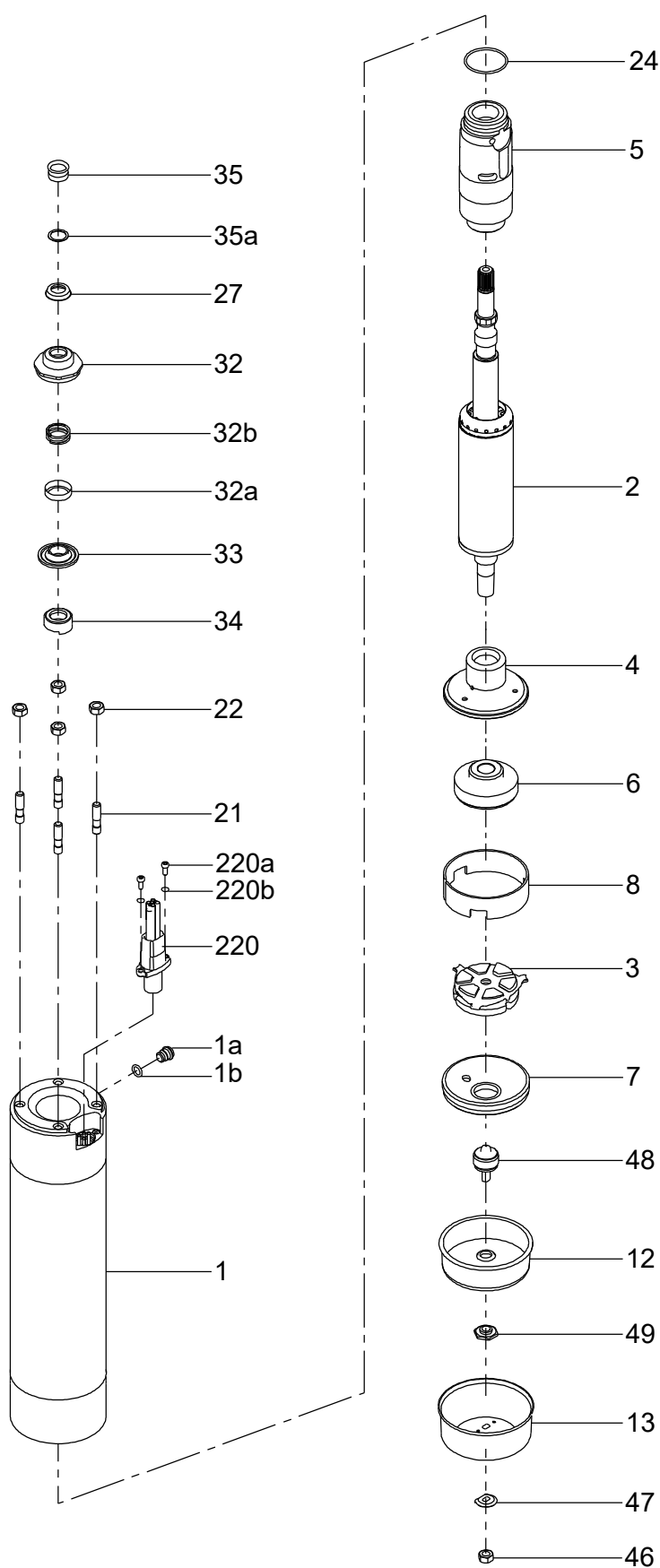
Exploded drawing of the MS4000 Model C motor
