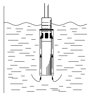
Flow sleeve function
