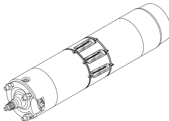
One anode string on the MS submersible motor
