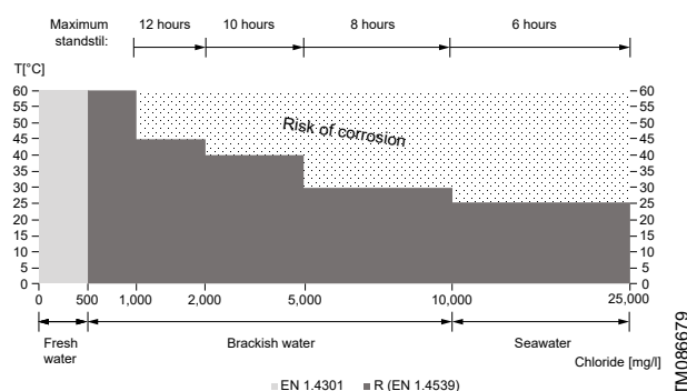
Corrosion resistance diagram at pH above 6.5
