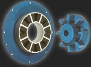
MULTI MONT OCTA flexible fly wheel couplings
