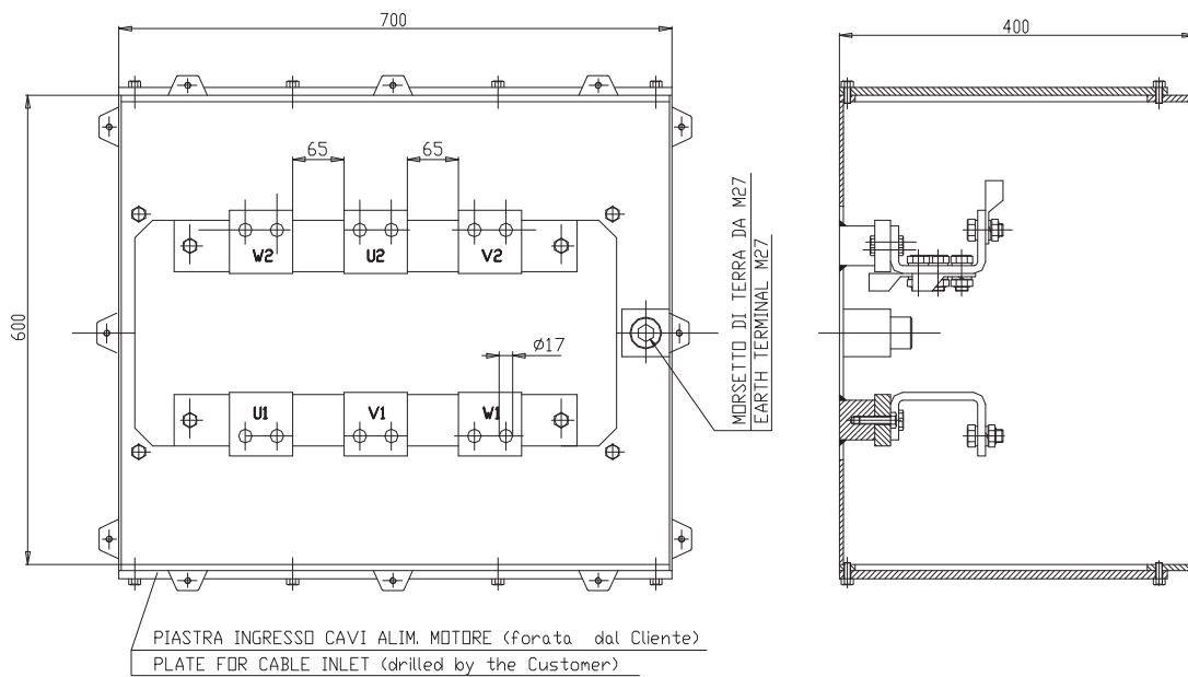
Morsetteria a 6 morsetti fornita con N. 3 piastre in rame per collegamento stella/triangolo Terminal block with 6 terminals supplied with Nr. 3 copper plates for star/delta connection
