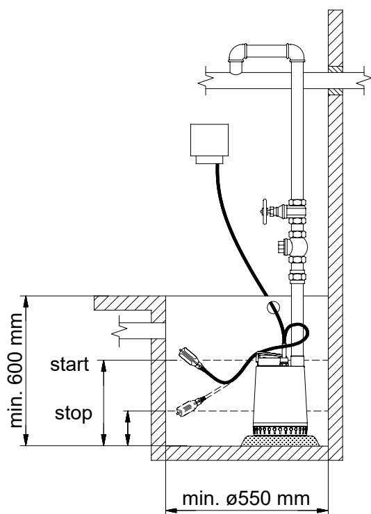
One-pump installation with float switch
