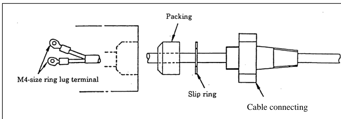
Figure 4.8 Cable connections
