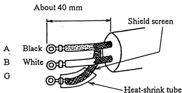
Figure 4.6 Termination of signal cable
