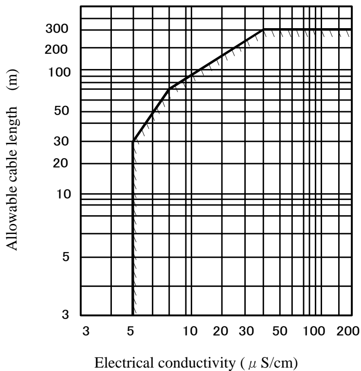
Figure 8.1 Electrical Conductivity vs. Cable Length
