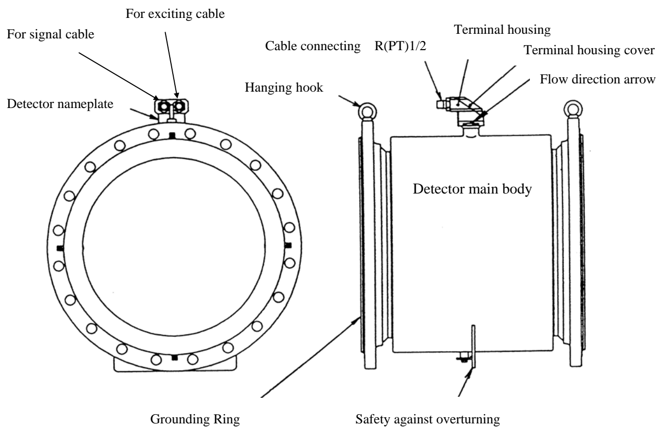
Figure 3.1 Outline drawing of the LF150 detector
