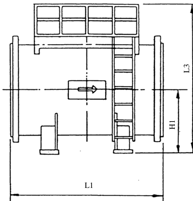
JIS 10K and AWWA class D dimensions:
