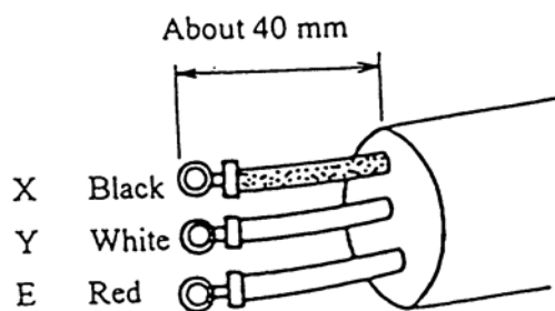
Figure 4.7 Termination of exciting cable
