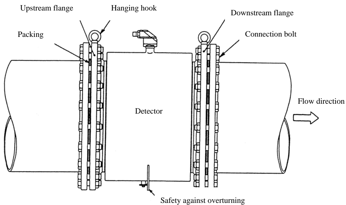
Figure 4.1 The LF150 detector piping connections
