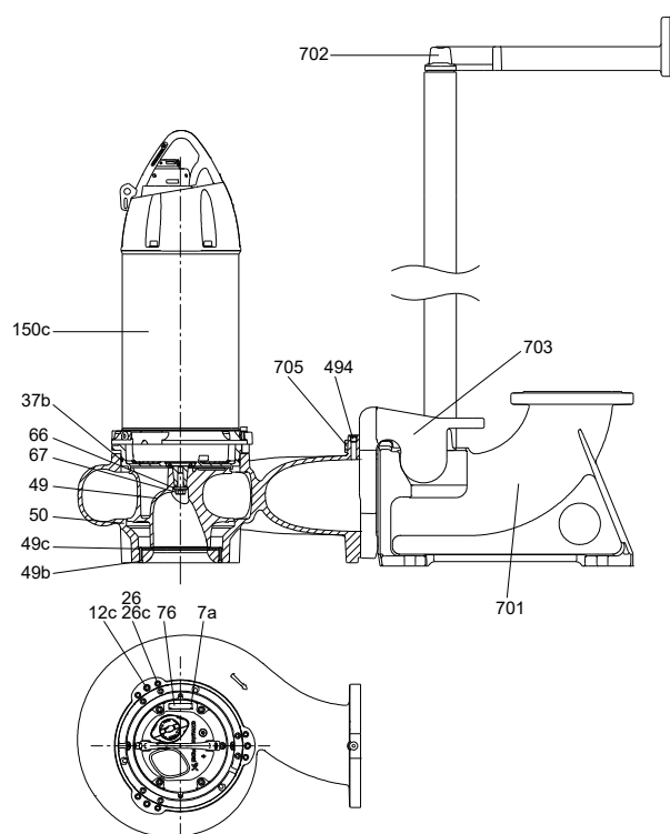
SE pump, with guide claw for auto-coupling
