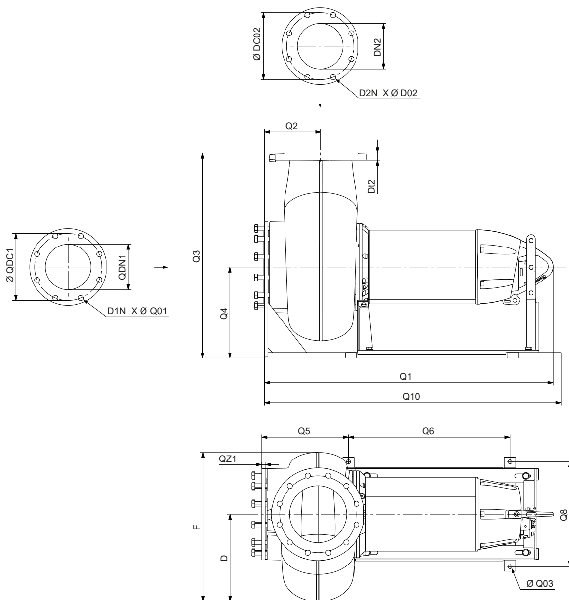
Horizontal base stand dimensions
