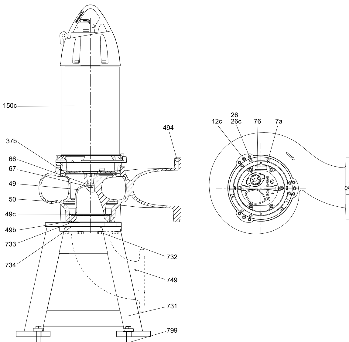
SE pump, dry installation on vertical base stand (recommended for SE pumps below 15 kW)
