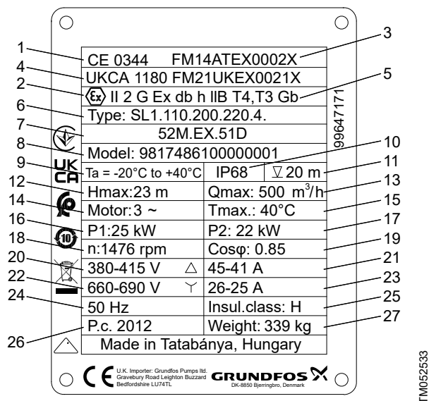
Nameplate example for Ex-proof pump
