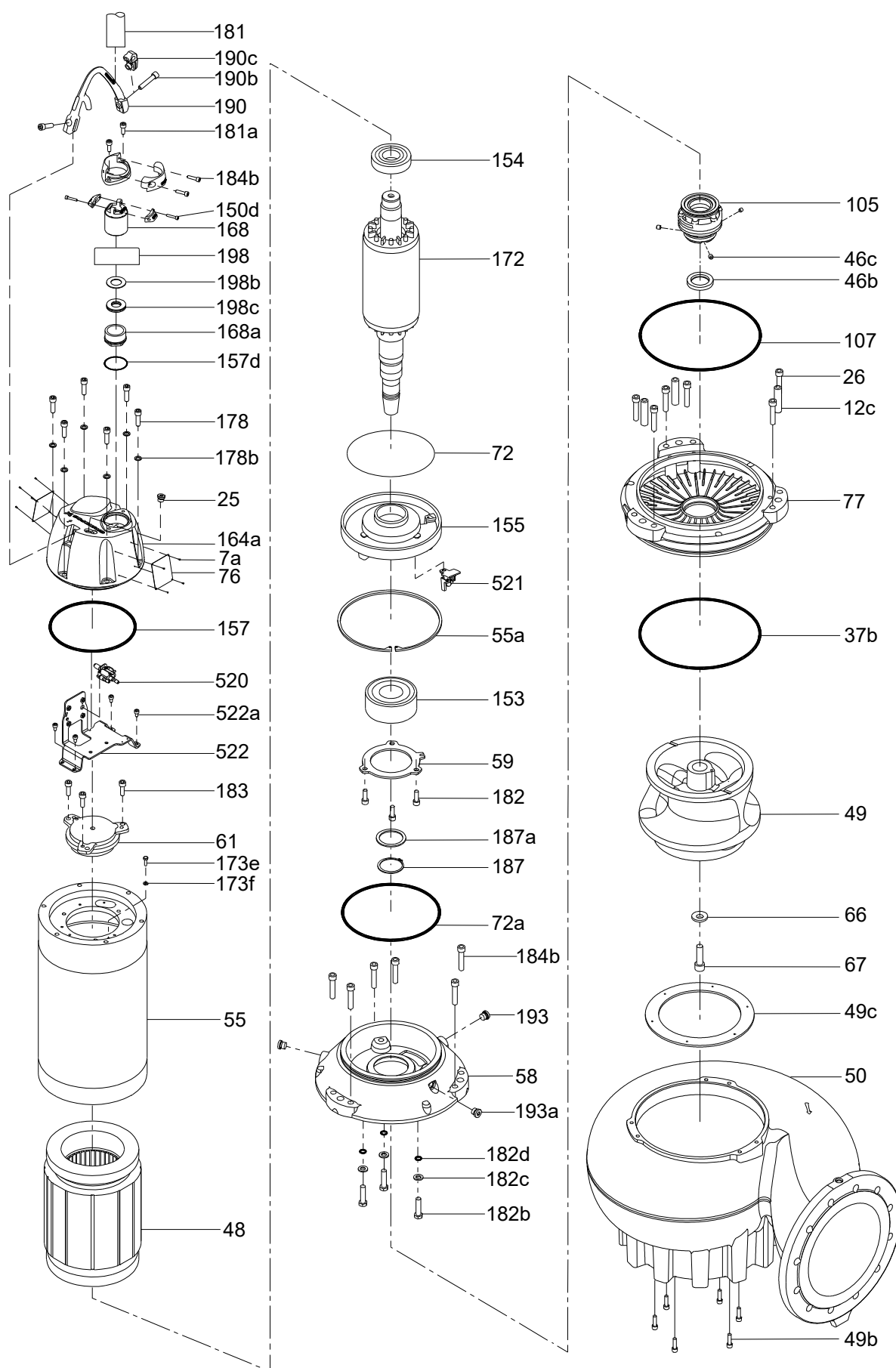
SL2 pumps, 6 poles
