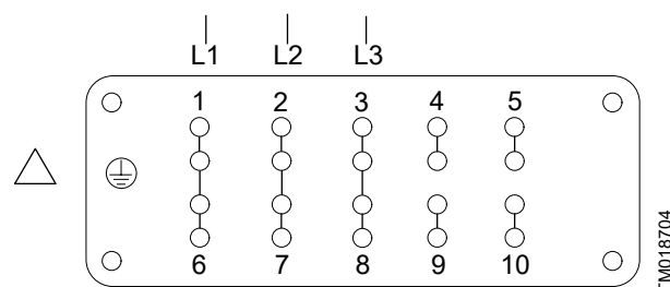
Plug connection for delta connection
