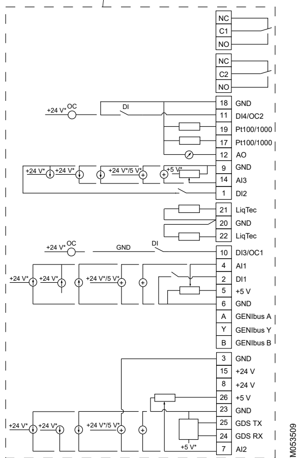
Connection terminals, FM300 functional module
