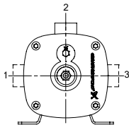
Alternative connection positions as seen from the pump inlet side
