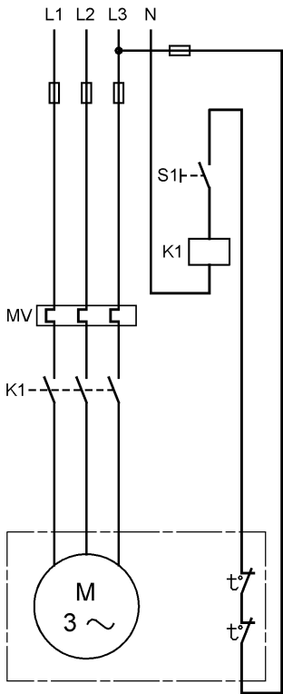
Three-phase motor with thermal switches
