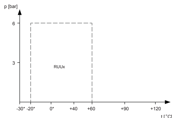
Curve for the RUUx shaft seal
