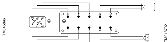
Plug connection from the motor
